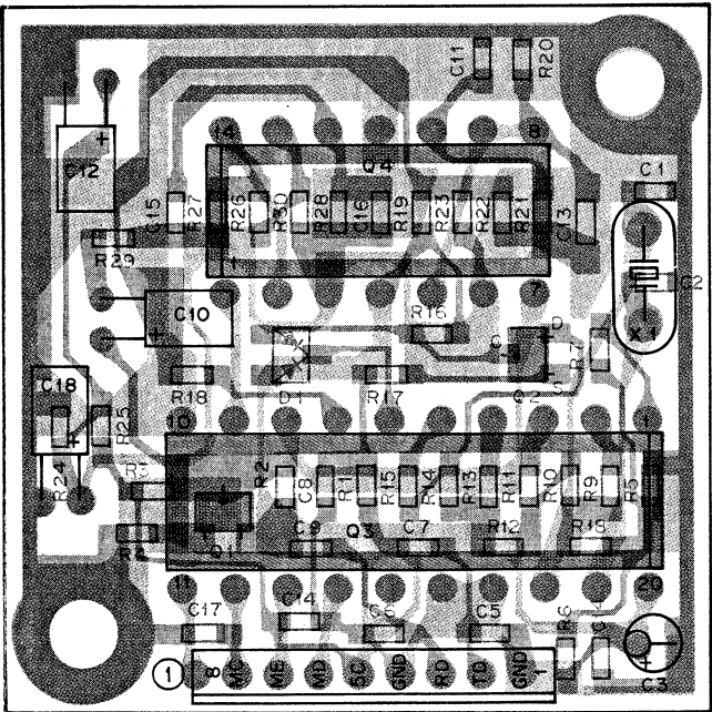
MU-1 PD BOARD VIEW (X57-1140-20) Component side view
